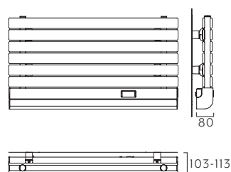
Piano Electric Horizontal
